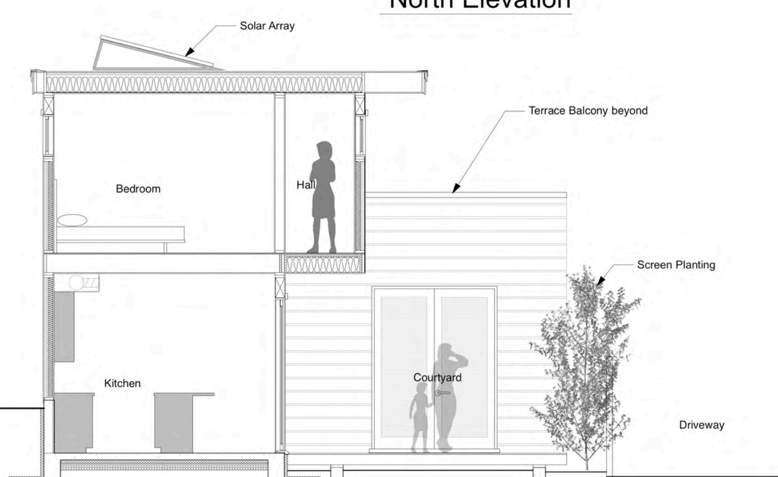
Building Section
